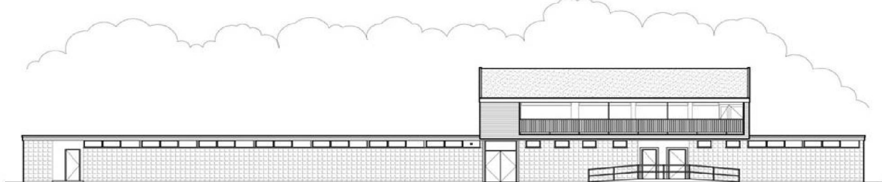
EXISTING ELEVATION B
